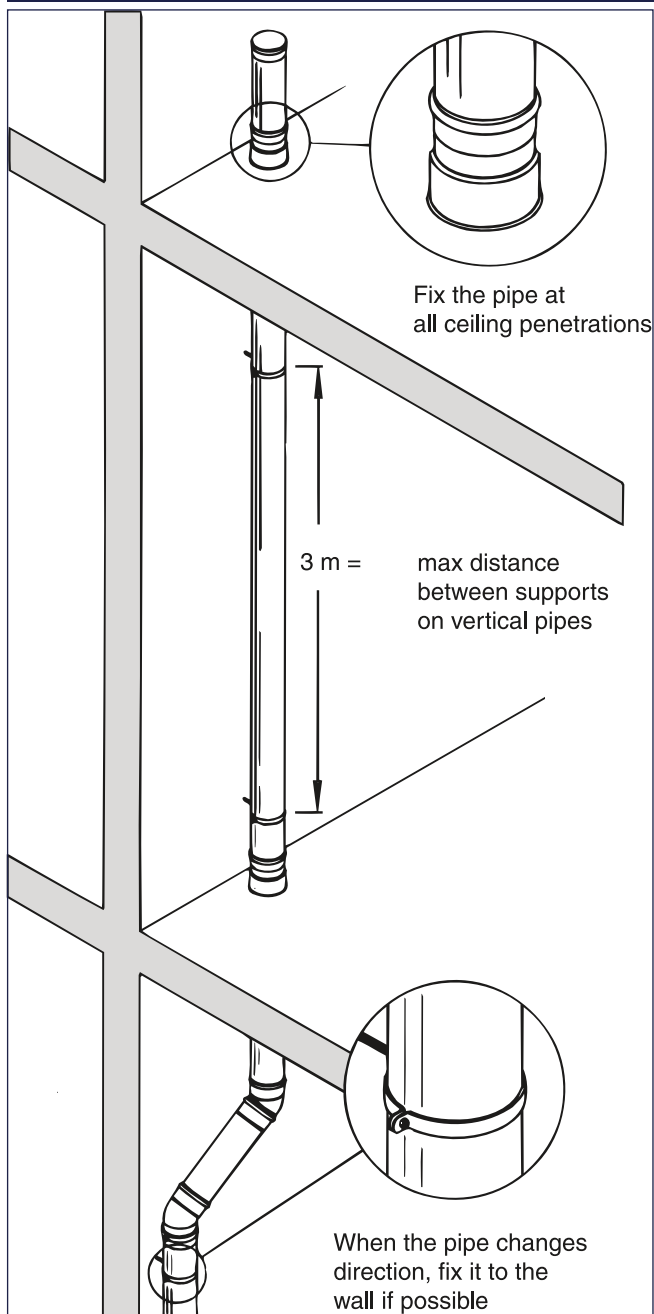
Vertical piping
